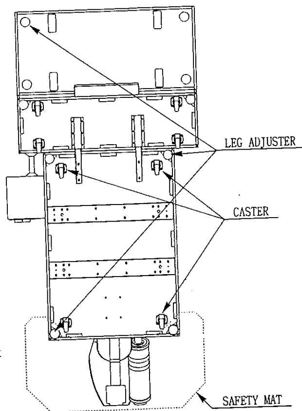
FIG. 6.4 a BOTTOM VIEW
